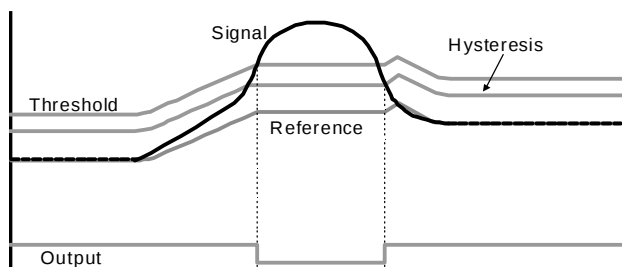
Figure 2.5 Drift Compensation
